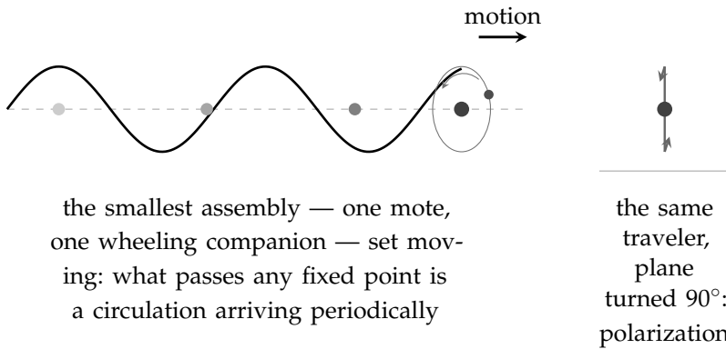
Figure 6.6.: Light, in the sketch: an object orbited by another, in motion — a particle doing a wave. The traveling pair is as localized as any particle and delivers its pushes in discrete arrivals; the pattern of those arrivals along the path is as periodic as any wave, with a frequency (the wheeling rate) and an orientation (the plane of the orbit). Turn the plane ninety degrees (right) and you have the other polarization — not a property bolted on, but geometry the object could not help having.
