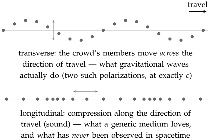
Figure 7.3.: The specification nature hands the layer below. If “space waving” is really the crowd below in motion, the crowd is not generic: its waves must be transverse only (top), in exactly two polarizations, at exactly the speed of light — and it must carry no longitudinal, sound-like mode (bottom), though ordinary media love nothing better. Add the Michelson–Morley demand that the crowd’s rest frame never show itself, and the reply to the gravitational-wave objection survives only as a very special crowd indeed.
