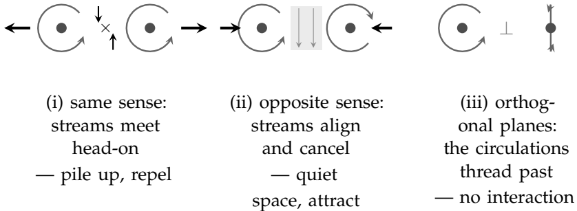
Figure 6.4.: Charge as circulation. Each charged assembly sheds circulating streams of its own substance. (i) Two assemblies circulating the same sense present head-on streams where they face each other: the streams pile up and the assemblies are pressed apart — like repels like. (ii) Opposite senses present aligned streams: they cancel, quiet the space between (shaded), and the shadow push does the rest — opposites attract, by the same mechanism as gravity but fiercer. (iii) Orbital planes at right angles neither pile nor cancel: the circulations pass through one another's business without transacting, as two crossed polarizing filters pass no common light.
